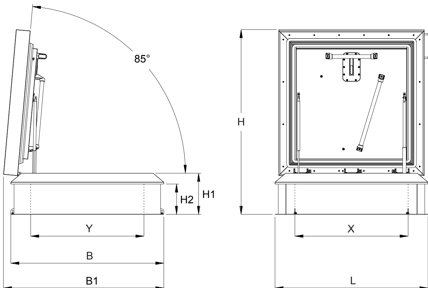
TopAccess dakluiken (in mm)
